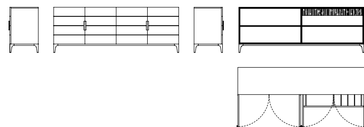
ML166 L2200 X H850 X P500MM APARADOR MILLER 4 PORTAS BUFFET MILLER 4 PORTES MILLER SIDEBOARD, 4 DOORS
